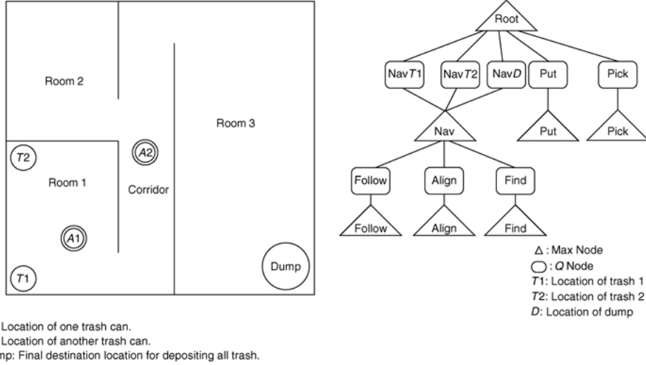
Figure 5. A two-robot (A1 and A2) trash collection task. The robots can learn to coordinate much more rapidly using the task structure than if they attempted to coordinate at the level of primitive movements. On the right is shown a MAXQ graph, which is MAXQ task graph with two kinds of nodes representing subtasks and the actions those subtasks can select. Reproduced from Makar et al. (2001) © 2001 ACM, Inc. Reprinted by permission.
